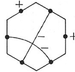
IH6 [3^6]
