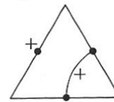
IH33 [3 . 6 . 3 . 6]
