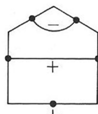
IH25 [3^3 . 4^2]
