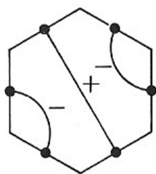
IH2 [3^6]
